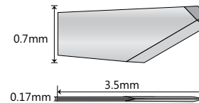
AK6150: Trifacet Available in: Angled, preset, and titanium
