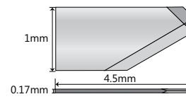
AK5015: 1.0mm trifacet freehand
