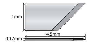
AK6026: 1.0mm 45 degree single edge Freehand
