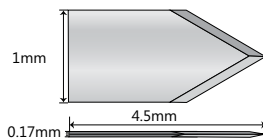
AK6035: 1.0mm freehand
