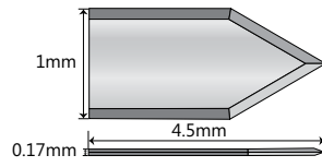
AK6216: 1.0mm clear cornea step handle
