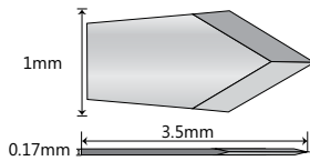
AK6175: 1.0mm lancet Available in: Angled, short handle, long handle, titanium, and preset
