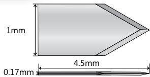
AK6235: 1.0mm lancet dull sides, step handle
